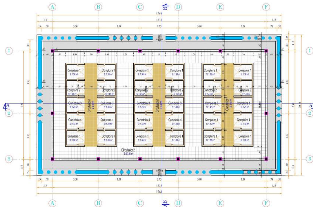
PLAN DE DISTRIBUTION - DISTRIBUTION PLAN
